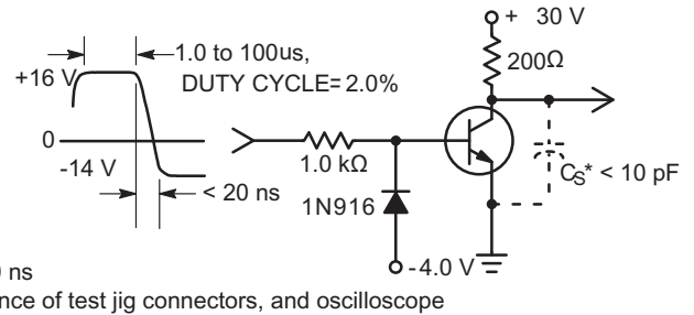
Figure 2. Turn-Off Time
