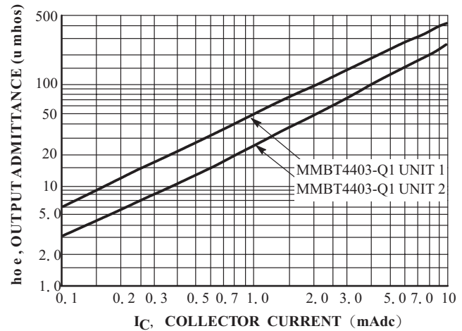
Figure 11. Output Admittance
