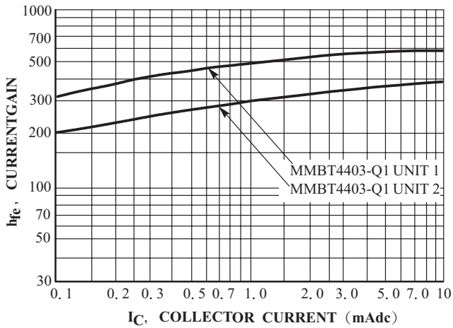
Figure 8. Current Gain
