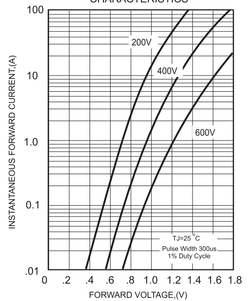
FIG.2-TYPICAL FORWARD CHARACTERISTICS
