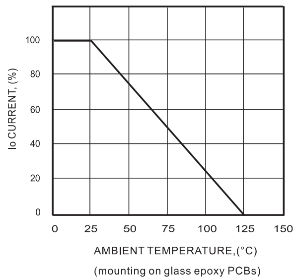
FIG.4- DERATING CURVE
