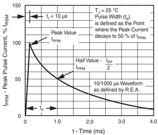
Fig. 3 - Pulse Waveform
