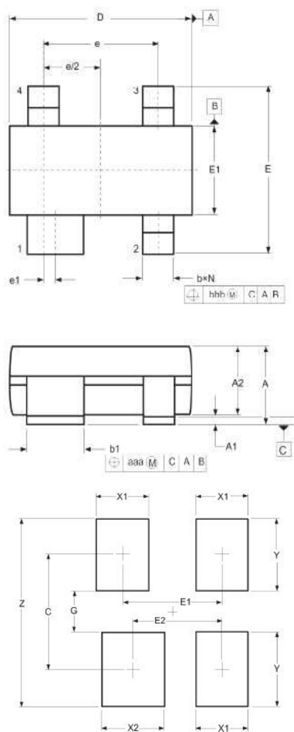
Land Pattern
