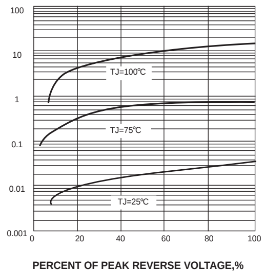
FIG. 4-TYPICAL REVERSE CHARACTERISTICS
